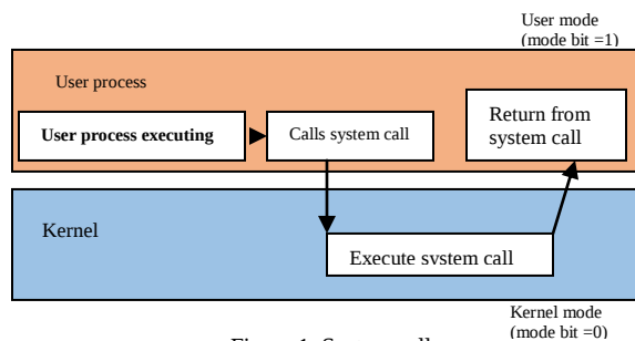
Figure 1. System calls
