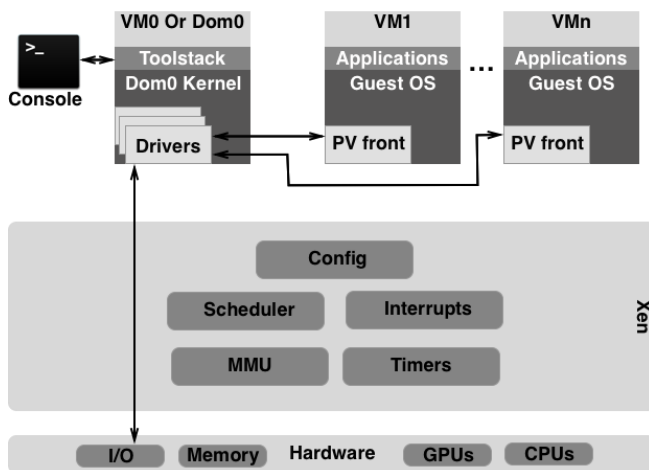
Figure 1. XEN Architecture.
