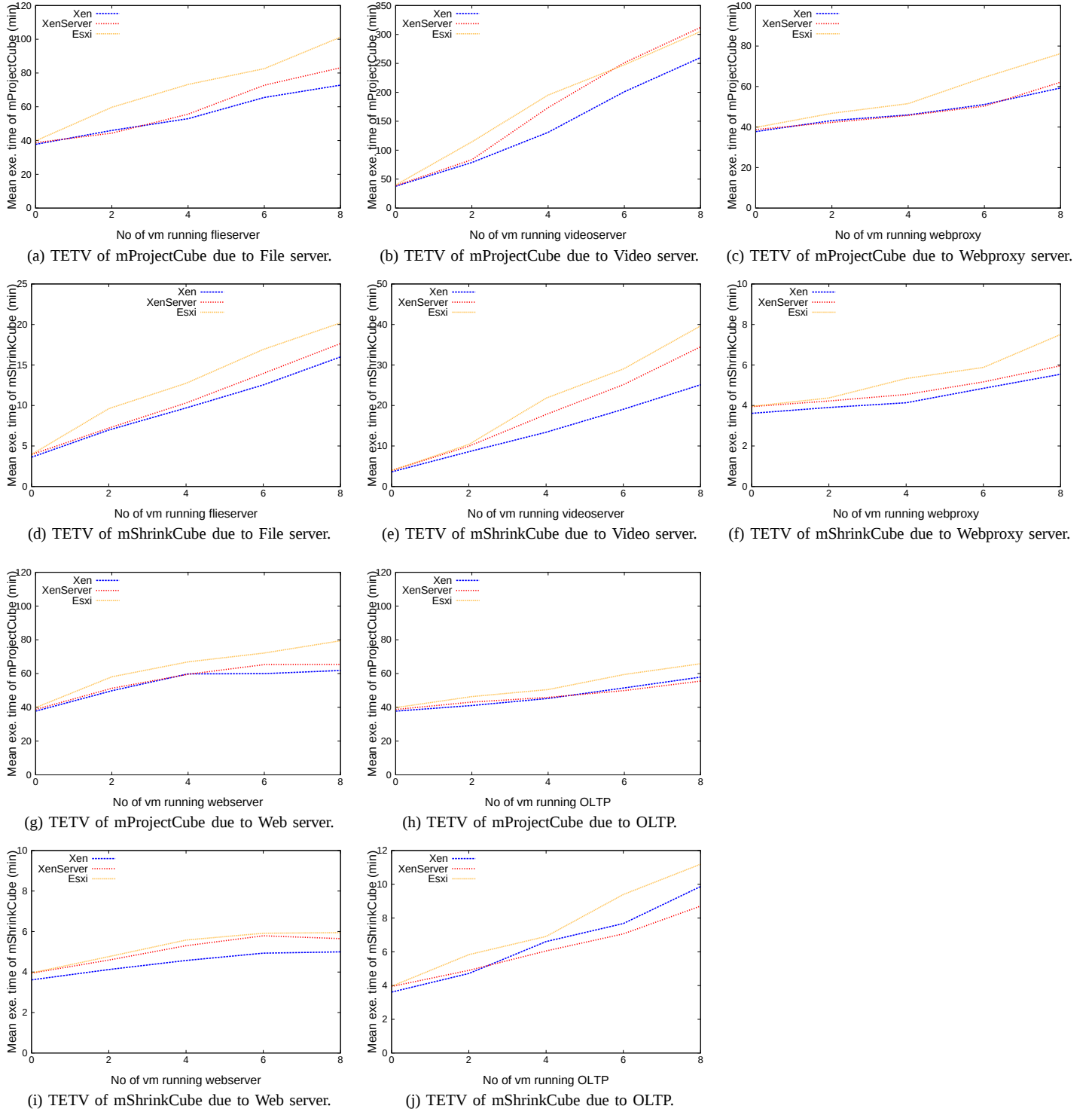
Figure 9. Task execution time variation (TETV) of the mProjectCube and mShrinkCube functions due to the I/O-intensive workload patterns on VMs.
