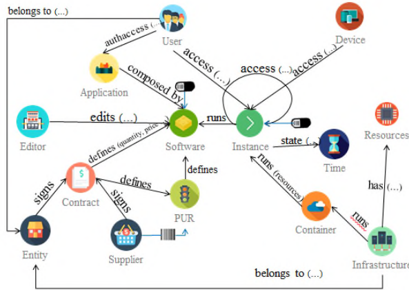
Figure 12. Graph modelization of SAM in Cloud
