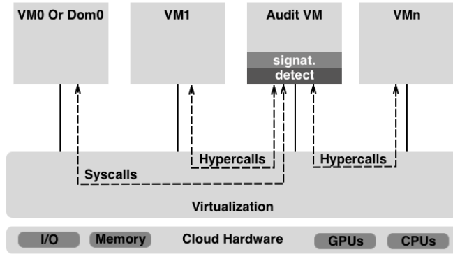
Figure 3. The MAD CROW Architecture.
