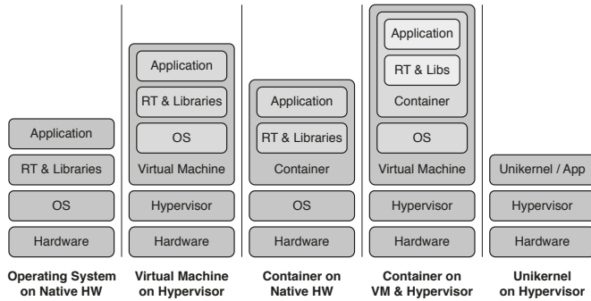
Figure 2. Illustrated comparison of the software stack complexity of various deployment strategies, including native setups, virtual machines, containers, containers within virtual machines and unikernels.
