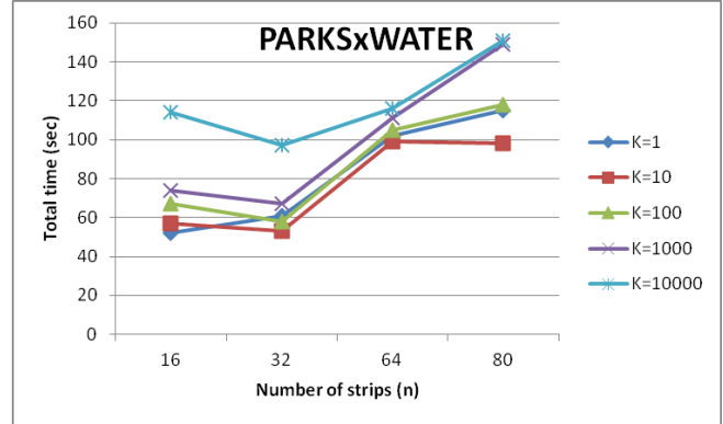
Figure 4. KCPQ (PARKS x WATER).
