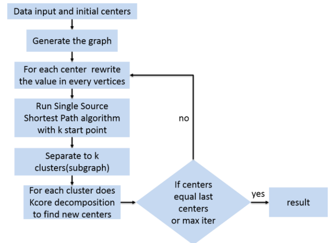
Figure 1. System flow chart.
