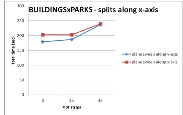
Figure 8. Split axis vs plane sweep axis.
