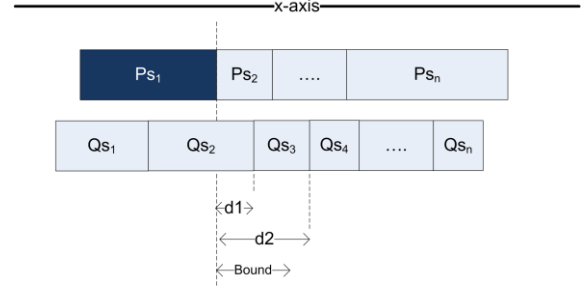
Figure 2. Eligible pairs of strips.
