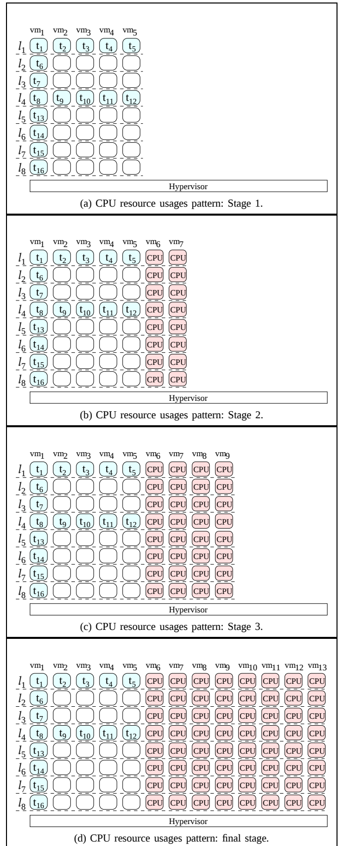
Figure 3. Applying CPU-intensive resource usages pattern on GALFA-HI workflow.
