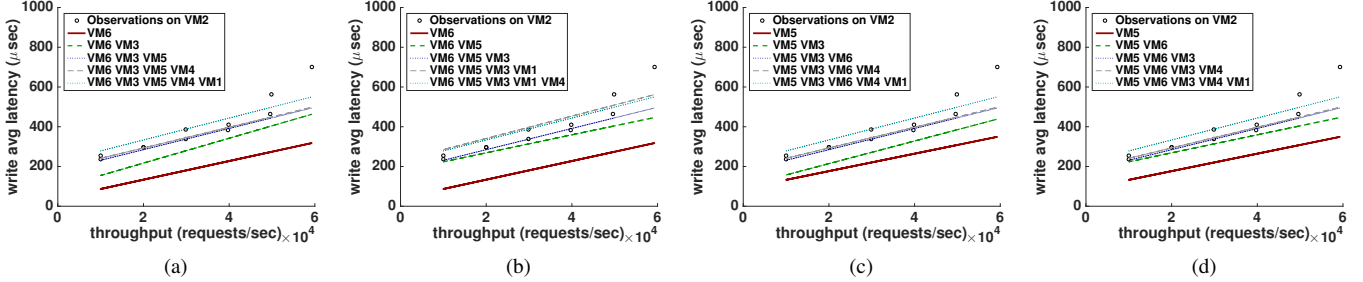
Fig. 4. Prediction of Redis write latency on VM_2 compared for model calibration using a variety of training sets ranging in size from 1 to 5 VM types.
