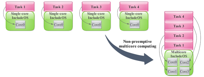
Figure 1. Multicore IncludeOS non-preemptive task management approach.
