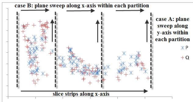
Figure 7. Strips Slice &amp; Plane Sweep cases.
