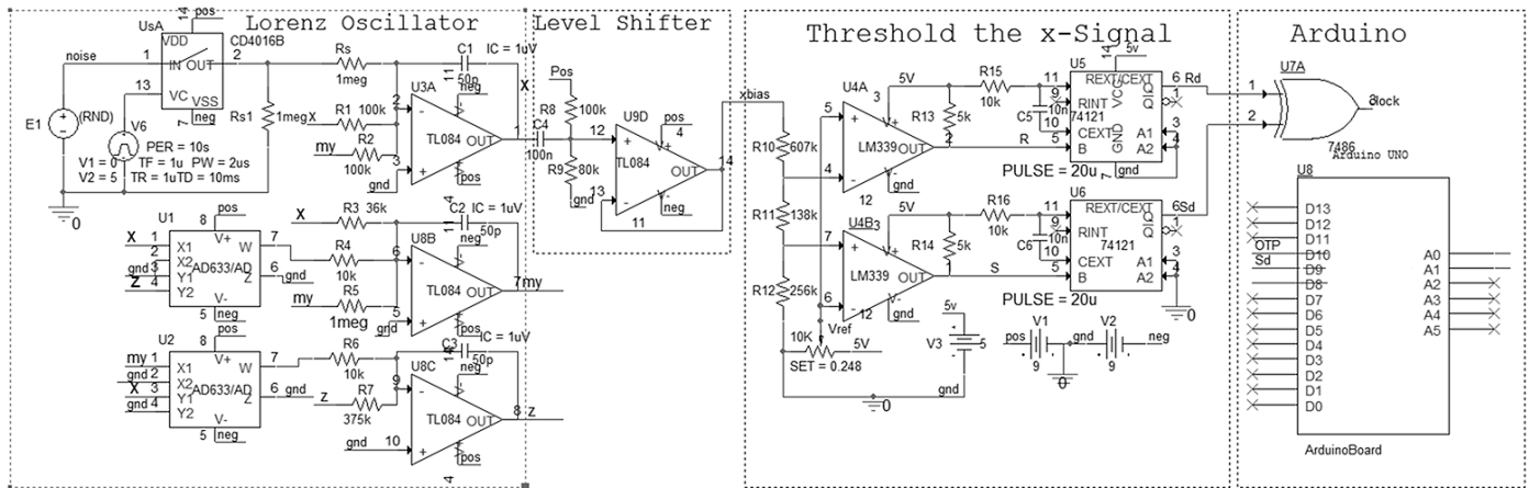
Figure 5. Generating the OTP.
