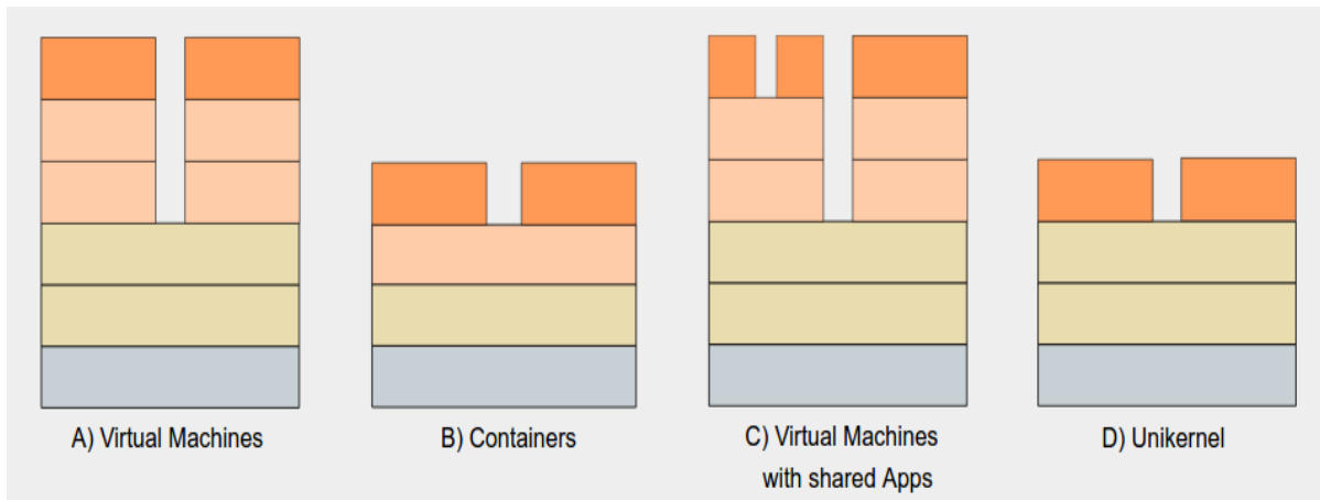
Fig. 1: A) Traditional virtual machines offer the highest level of service isolation but introduce high overhead as each application should—theoretically—be placed within a virtual machine of its own. B) Containers improve efficiency by reusing large parts of the host operating system and kernel, but are thus not able to provide the security guarantees of fully separated virtual machines, e.g., resource starvation as well as kernel-level exploits can have cross-container impact. C) A new trend is to encapsulate one or more containers into virtual machines on their own. This improves security and service isolation but introduces the overhead of virtual machine based solutions. D) Unikernels, in contrast, are minimal virtual machines thus yield the high security assumptions of virtual machine based approaches while improving efficiency through their minimalism.
