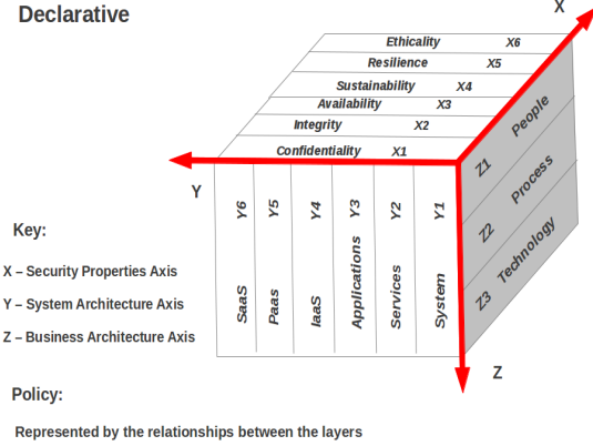
Fig. 1. A Declarative Cloud Three-Dimensional Security Matrix
