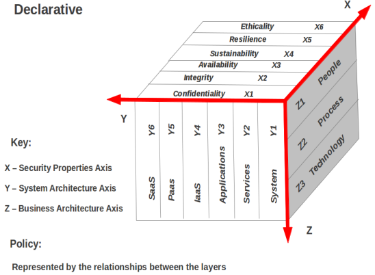
Fig. 2. A Declarative Cloud Three-Dimensional Security Matrix
